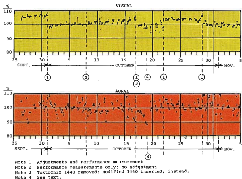
Fig. 5 WNJT-TV POWER OUTPUT STABILITY
