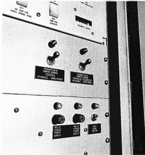
Monitoring and status displays for KNTV transmitter operation. Lower panel is logic system for RF switching sequences. The panel above this displays the "Summation of Control Data" referred to in text.
